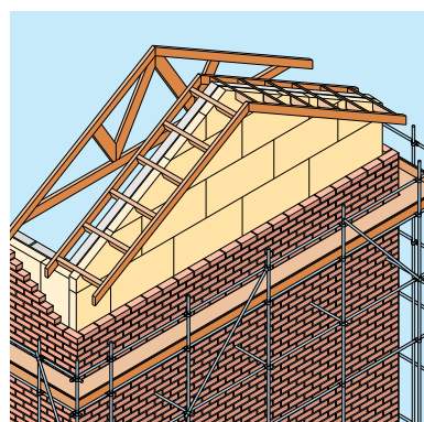
Figure 6 Installation of Batts in gable end wall
